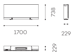
Closed module
