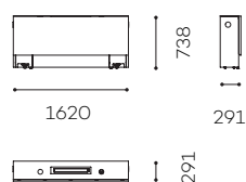
Closed module
